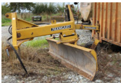
Farmgrad 3PTL Grader Blade-Hydraulic Adjustment
