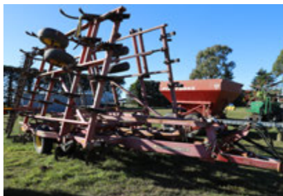
Sunflower Cultivator
